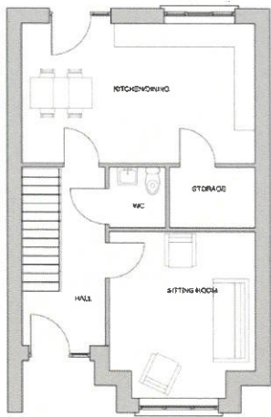
HOUSE LAYOUT A SEMI-DETACHED 3 BEDROOM HOUSE WITH MASTER ENSUITE 105 SQ MTS
