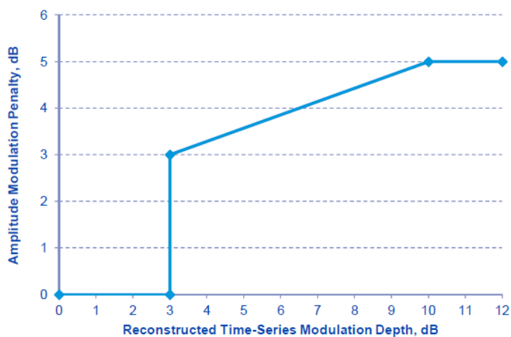
Figure 2.1: UK DECC Proposed AM Level Penalty Scheme
