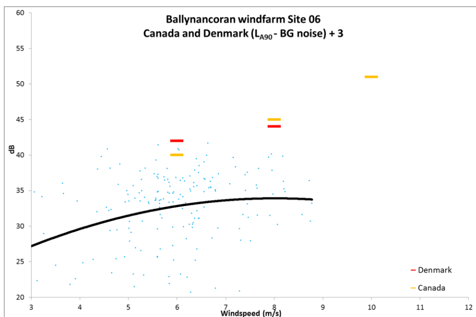
Figure 6.23: Site 06 L_{A90} minus BG noise + 3dB data against Danish guidelines
