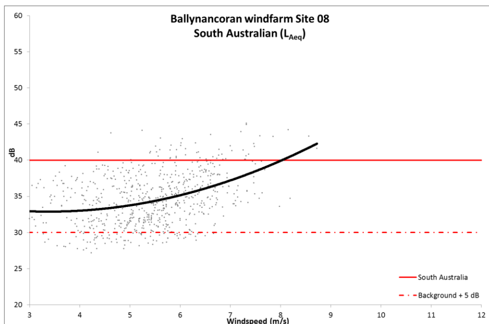
Figure 6.16: Site 08 L_{Aeq} data against background noise levels and South Australian guidelines
