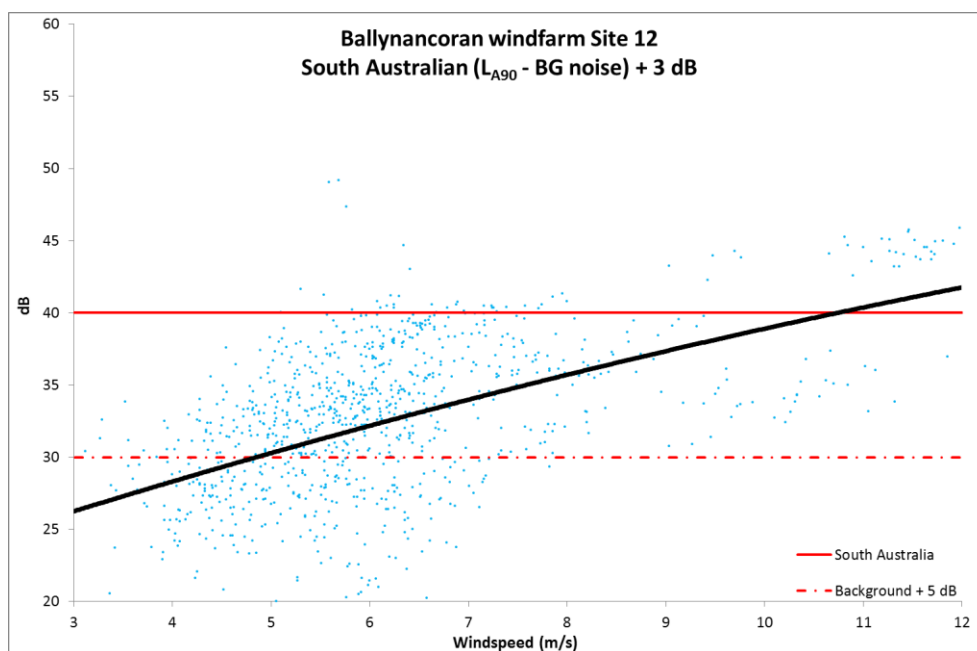
Figure 6.19: Site 12 Corrected L_{A90} against South Australian guidelines
