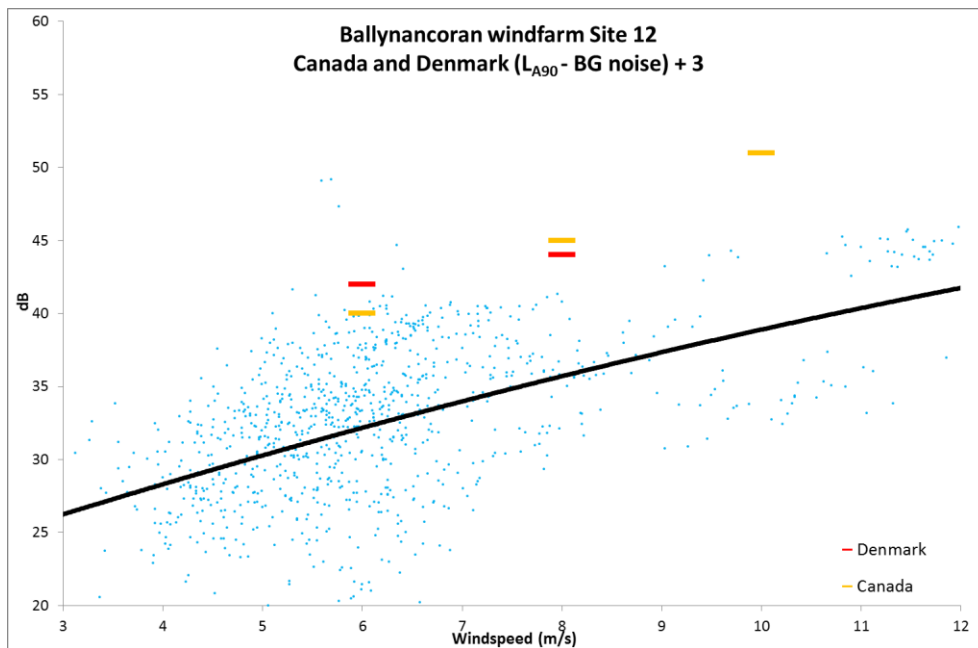
Figure 6.29: Site 12 L_{A90} minus BG noise + 3dB data against Danish guidelines
