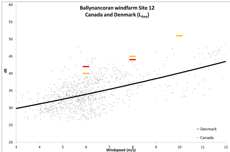
Figure 6.28: Site 12 L_{Aeq} data against Danish guidelines
