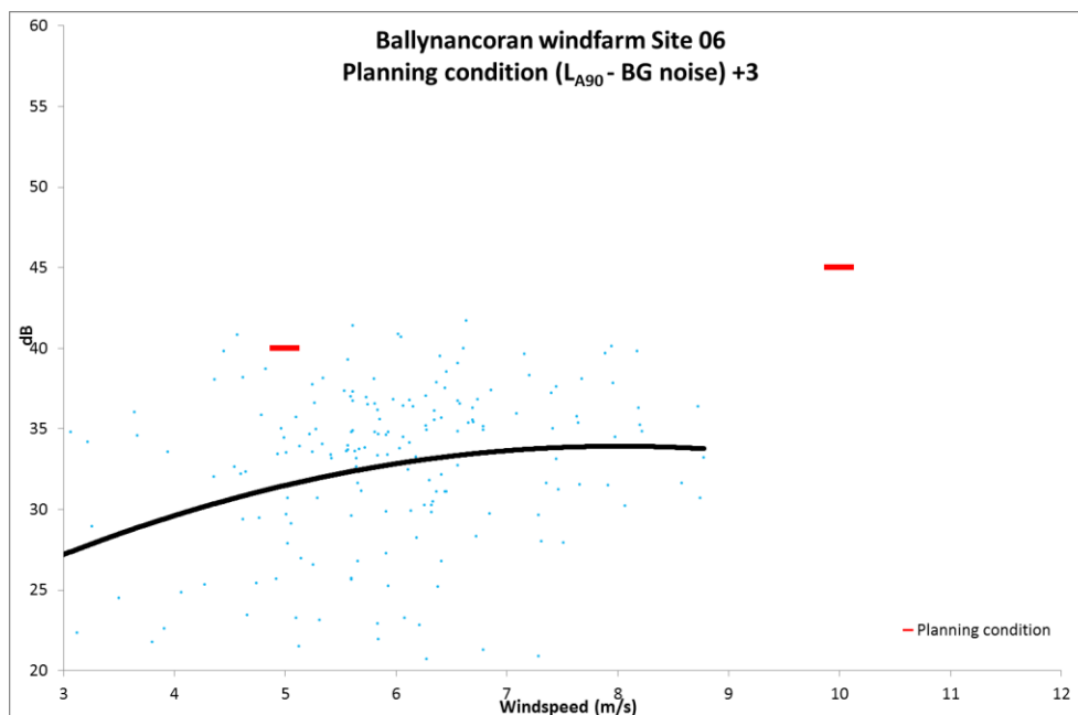
Figure 6.3: Site 06 – Compliance with Planning Condition 15 Limits
