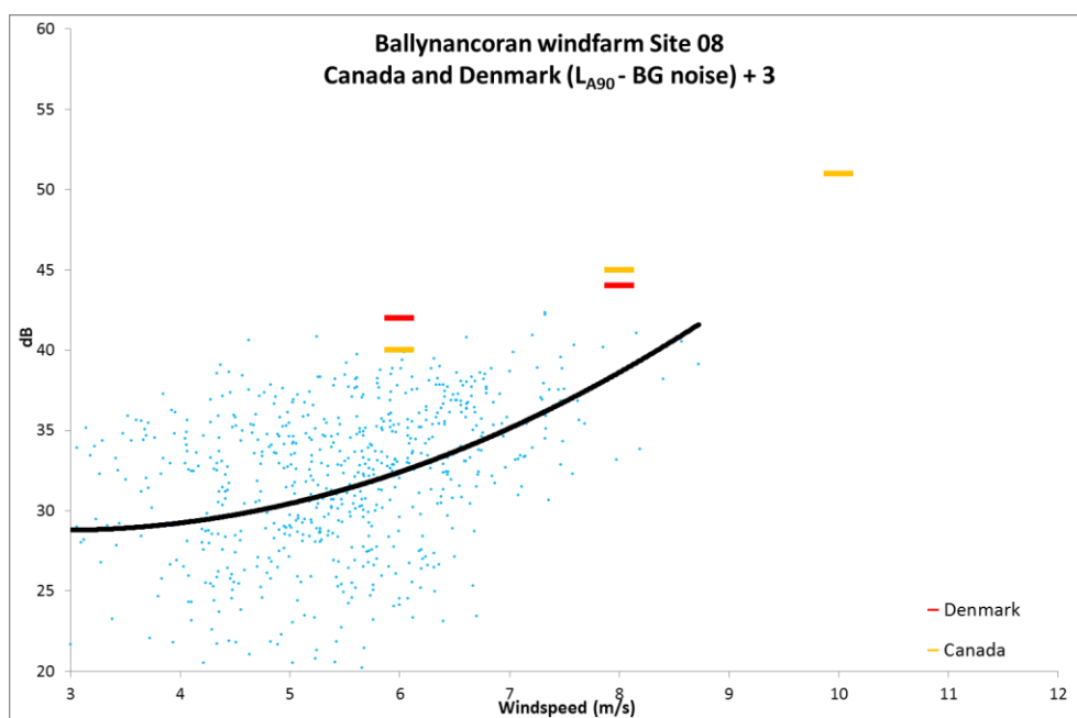
Figure 6.27: Site 08 L_{A90} minus BG noise + 3dB data against Danish guidelines
