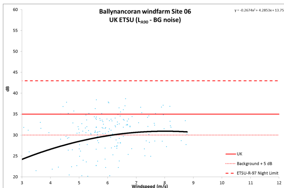
Figure 6.7: Site 06 Corrected L_{A90} against UK ETSU guidelines
