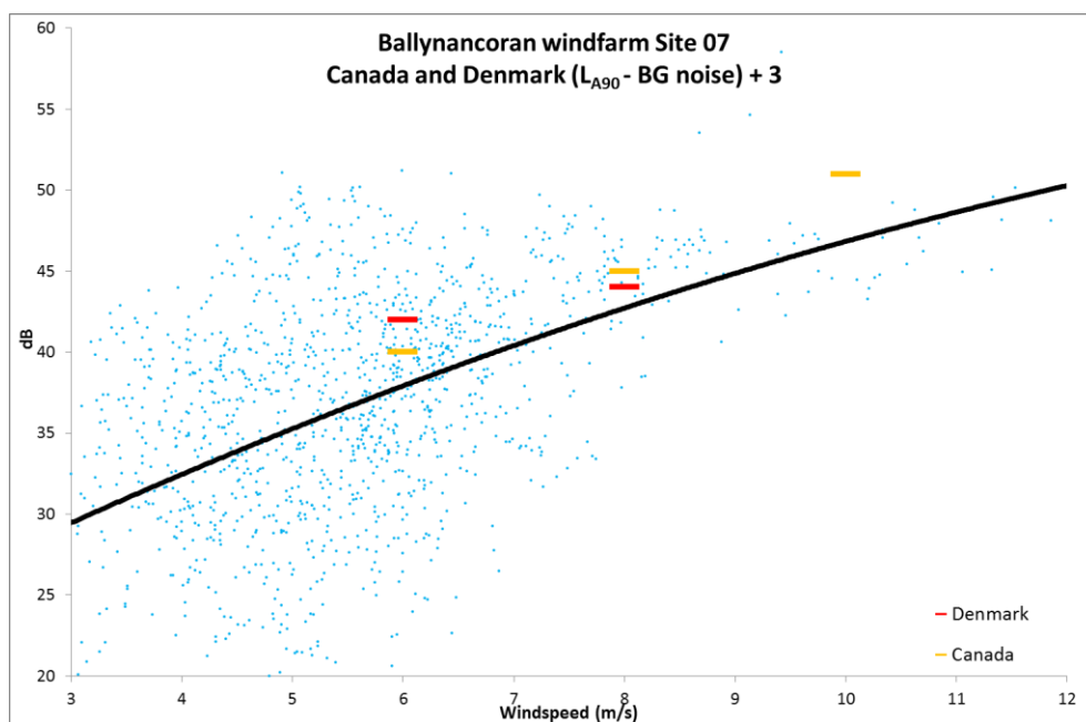
Figure 6.25: Site 07 L_{A90} minus BG noise + 3dB data against Danish guidelines
