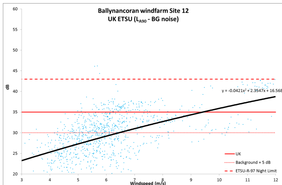
Figure 6.10: Site 12 Corrected L_{A90} against UK ETSU guidelines
