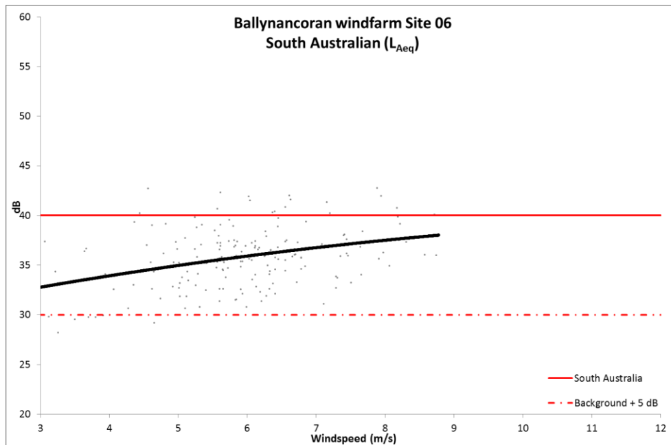
Figure 6.12: Site 06 L_{Aeq} data against background noise levels and South Australian guidelines
