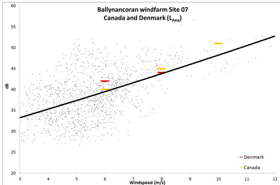
Figure 6.24: Site 07 L_{Aeq} data against Danish guidelines
