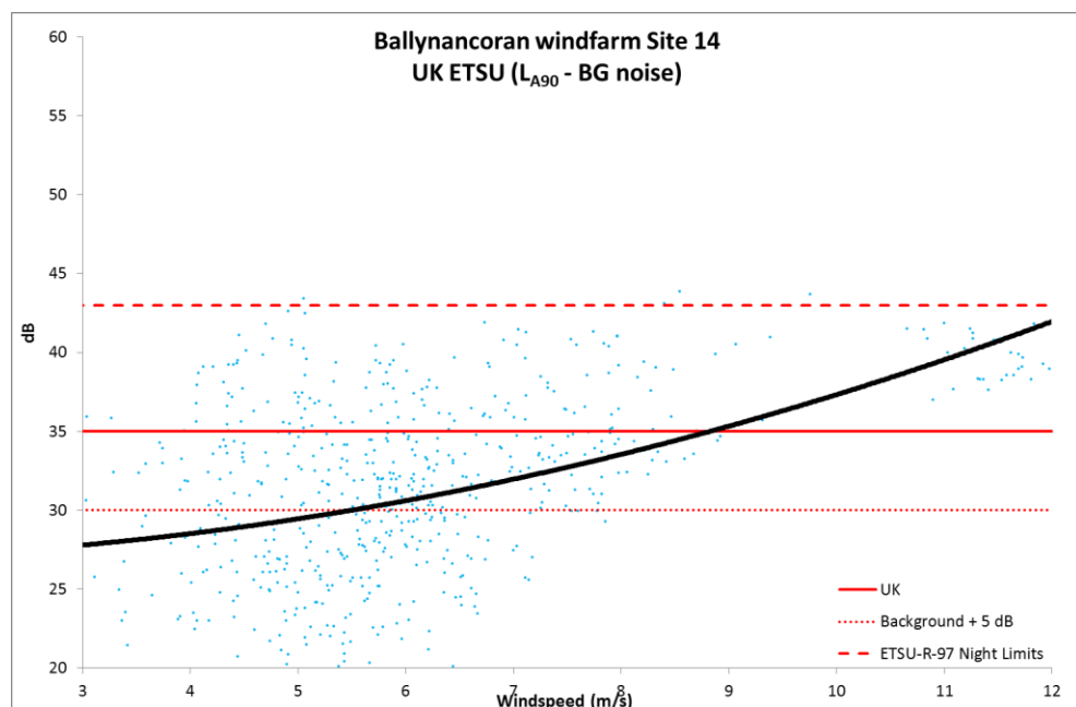
Figure 6.11: Site 14 Corrected L_{A90} against UK ETSU guidelines
