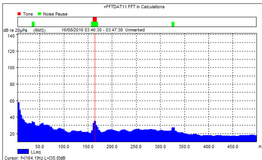
Figure 6.32 FFT Analysis Plot
