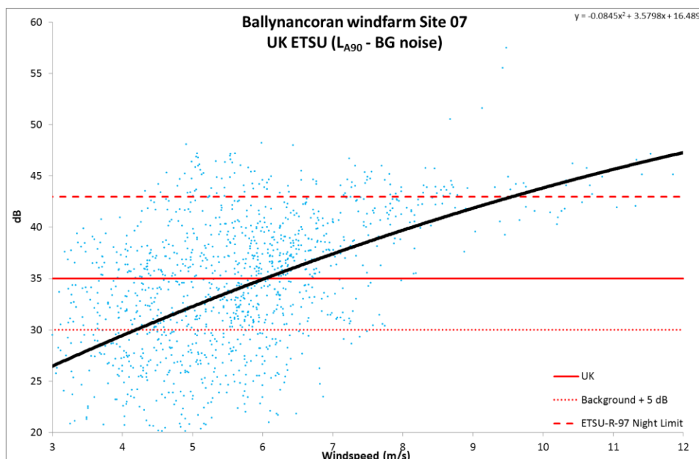
Figure 6.8: Site 07 Corrected L_{A90} against UK ETSU guidelines
