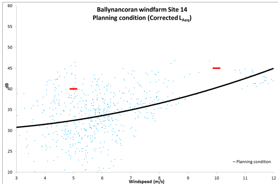
Figure Site 14 – Compliance with Planning Condition 15 Limits
