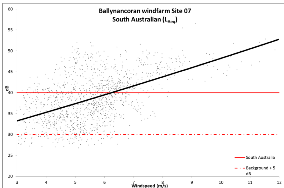
Figure 6.14: Site 07 L_{Aeq} data against background noise levels and South Australian guidelines
