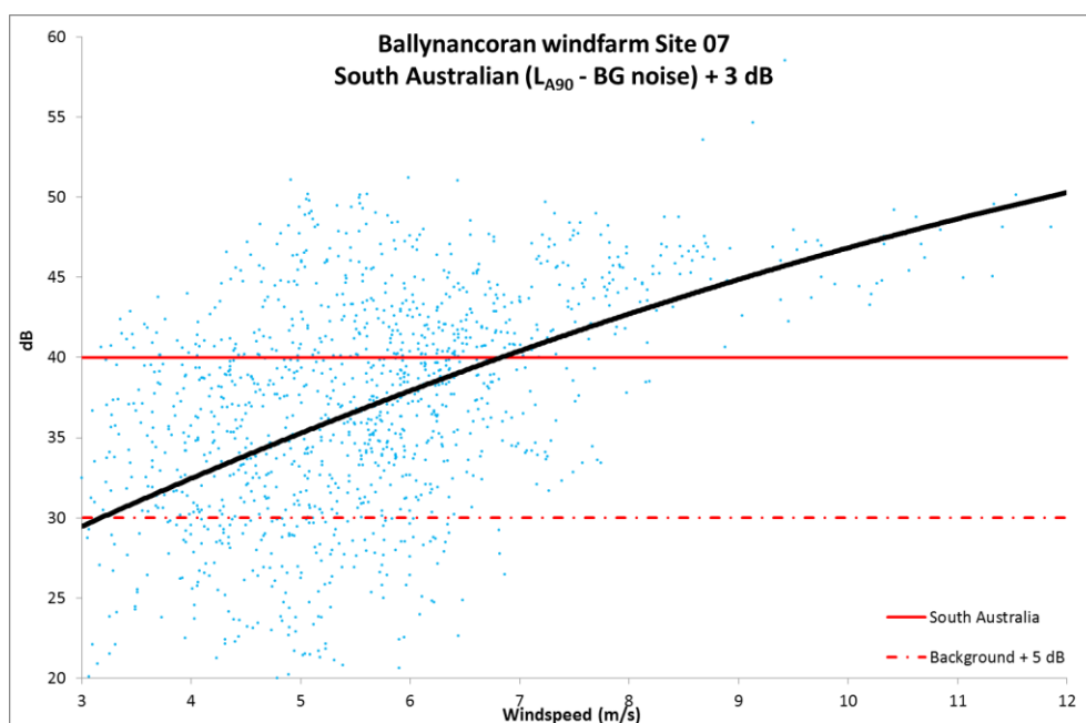
Figure 6.15: Site 07 Corrected L_{A90} against South Australian guidelines
