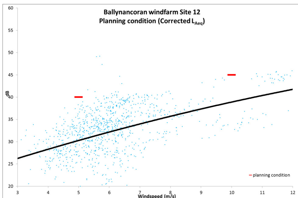
Figure 6.6: Site 12 – Compliance with Planning Condition 15 Limits
