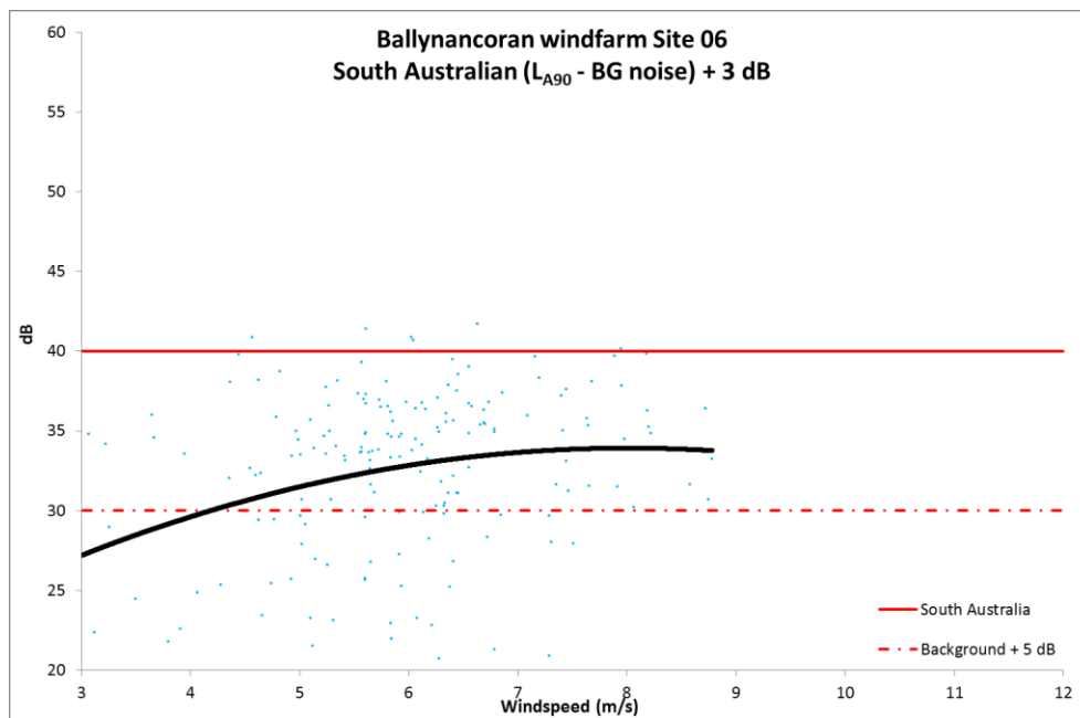
Figure 6.13: Site 06 Corrected L_{A90} against South Australian guidelines
