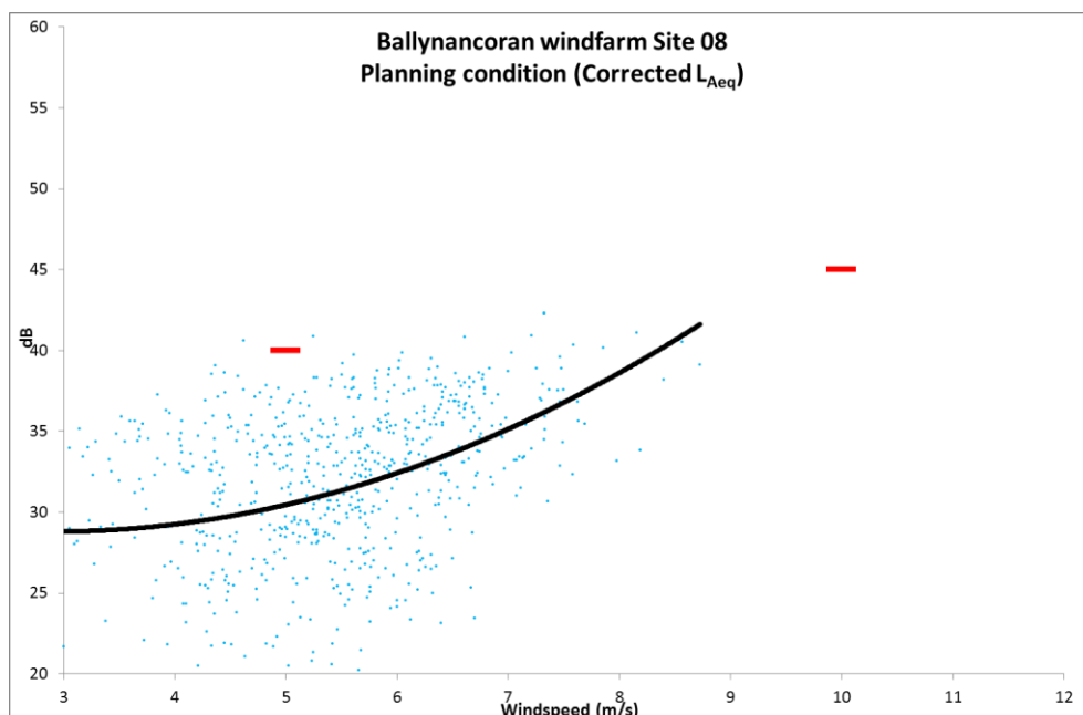
Figure 6.5: Site 08 – Compliance with Planning Condition 15 Limits
