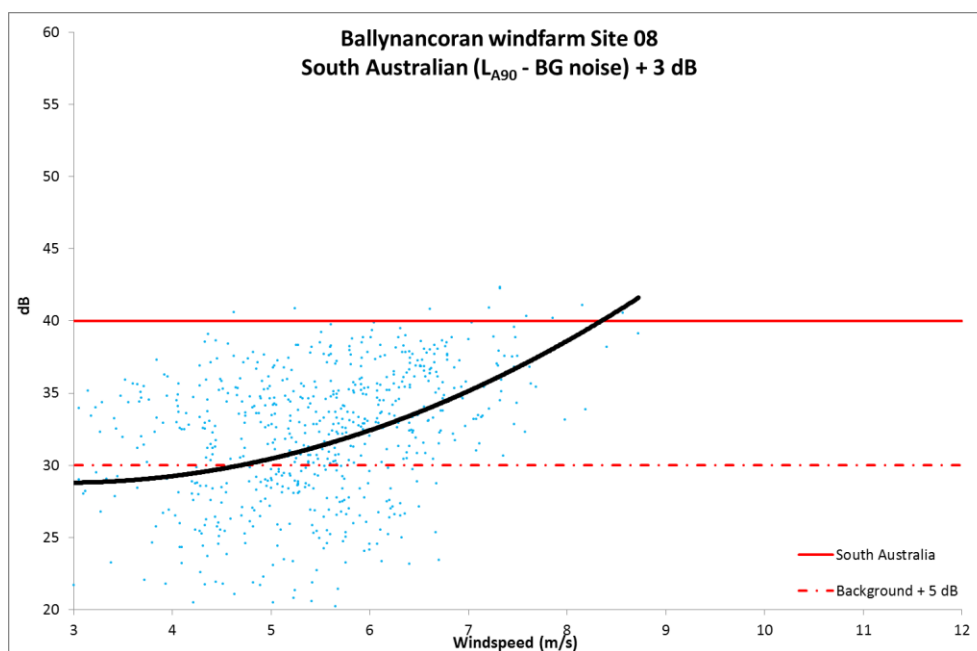
Figure 6.17: Site 08 Corrected L_{A90} against South Australian guidelines
