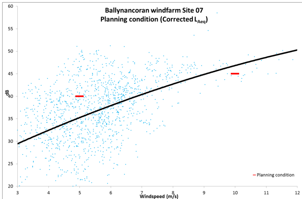
Figure 6.4: Site 07 – Compliance with Planning Condition 15 Limits
