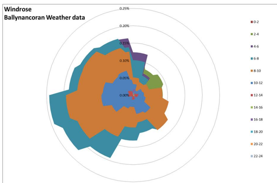
Figure 6.2: Windrose of Ballynancoran weather data (all turbines all time)
