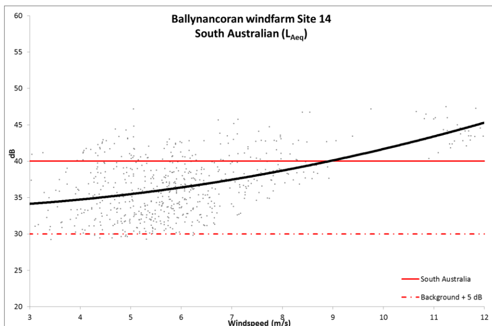
Figure 6.20: Site 14 L_{Aeq} data against background noise levels and South Australian guidelines
