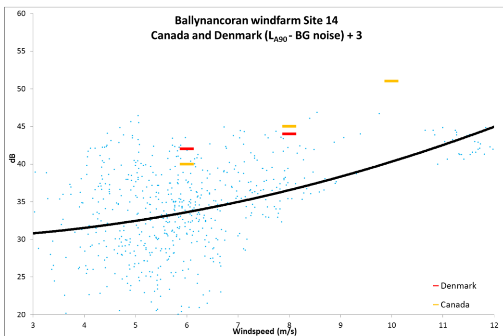
Figure 6.31: Site 14 L_{A90} minus BG noise + 3dB data against Danish guidelines
