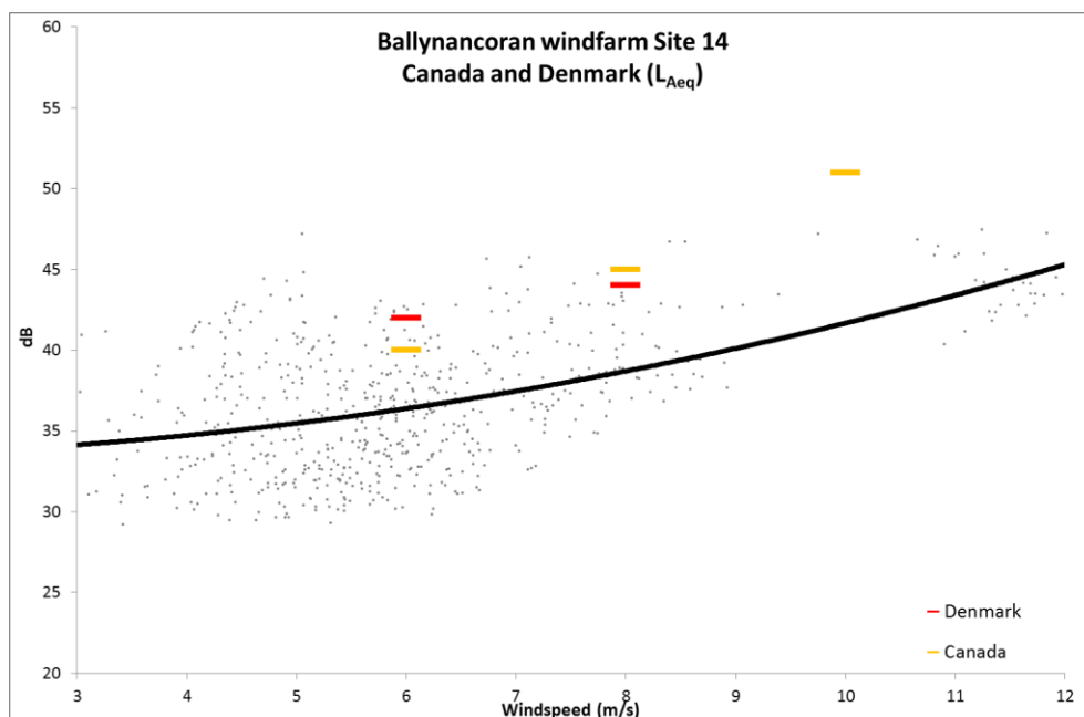
Figure 6.30: Site 14 L_{Aeq} data against Danish guidelines
