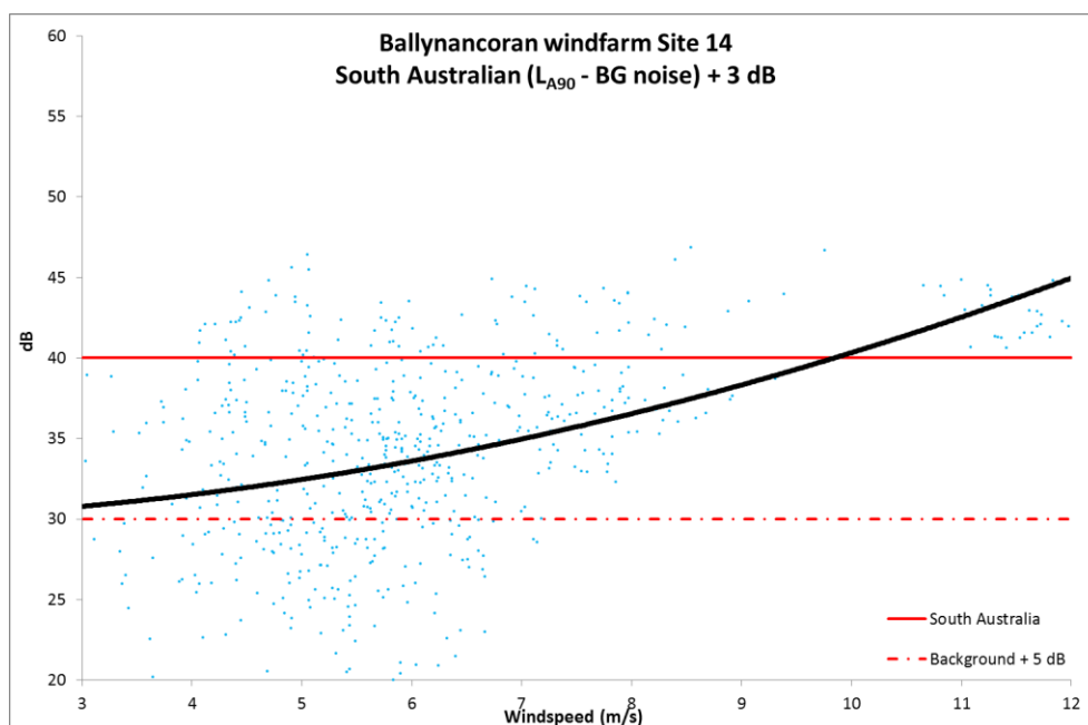
Figure 6.21: Site 14 Corrected L_{A90} against South Australian guidelines
