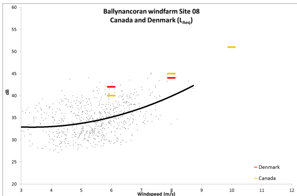
Figure 6.26: Site 08 L_{Aeq} data against Danish guidelines
