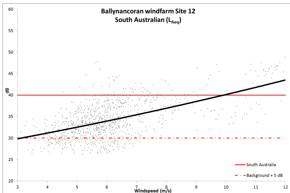
Figure 6.18: Site 12 L_{Aeq} data against background noise levels and South Australian guidelines
