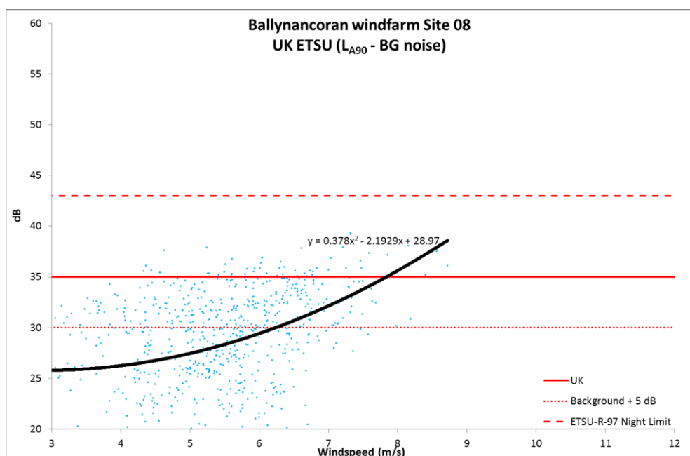
Figure 6.9: Site 08 Corrected L_{A90} against UK ETSU guidelines
