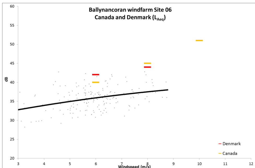
Figure 6.22: Site 06 L_{Aeq} data against Danish guidelines
