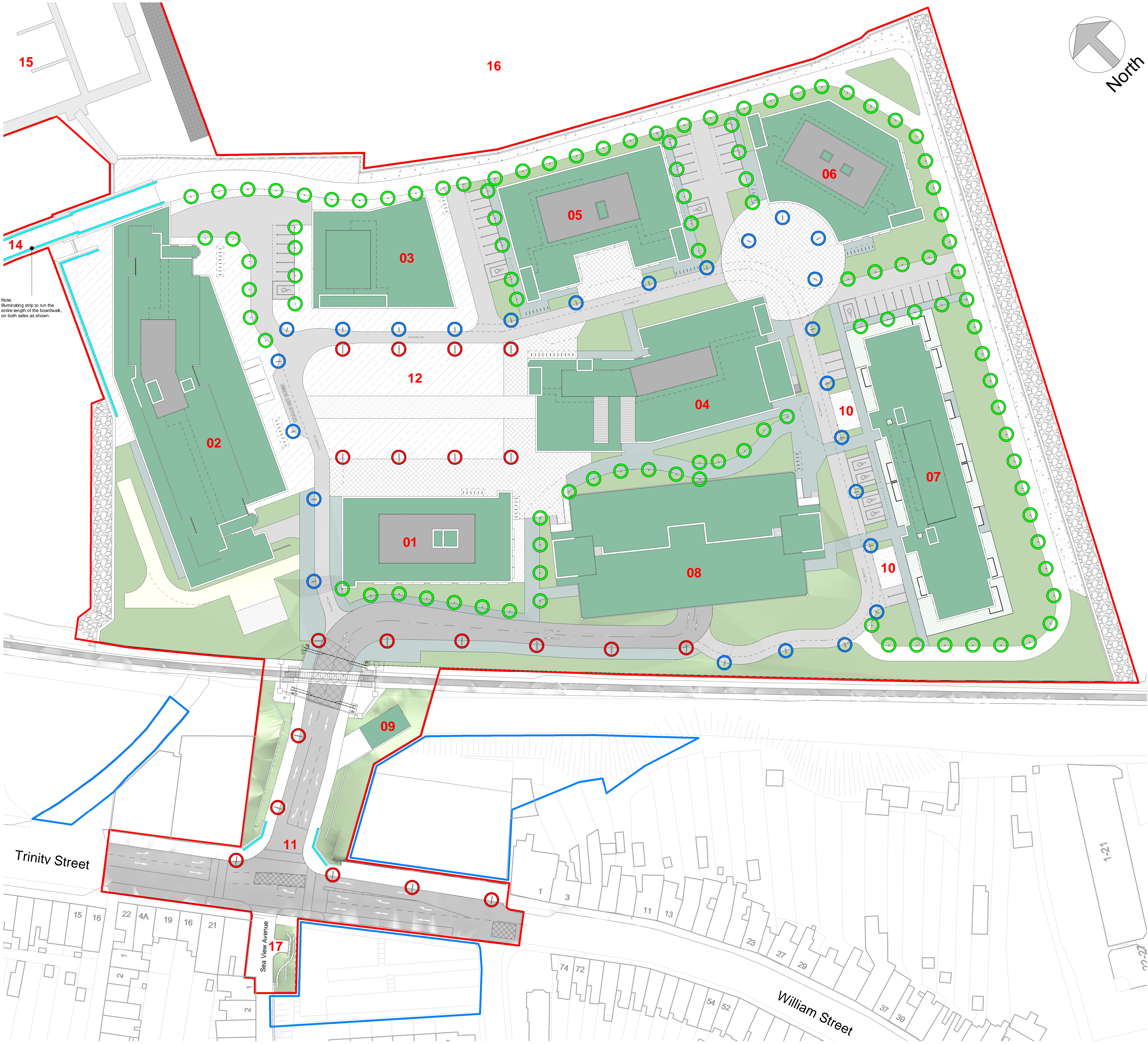
1-PROPOSED SITE LAYOUT - EXTERNAL LIGHTING
