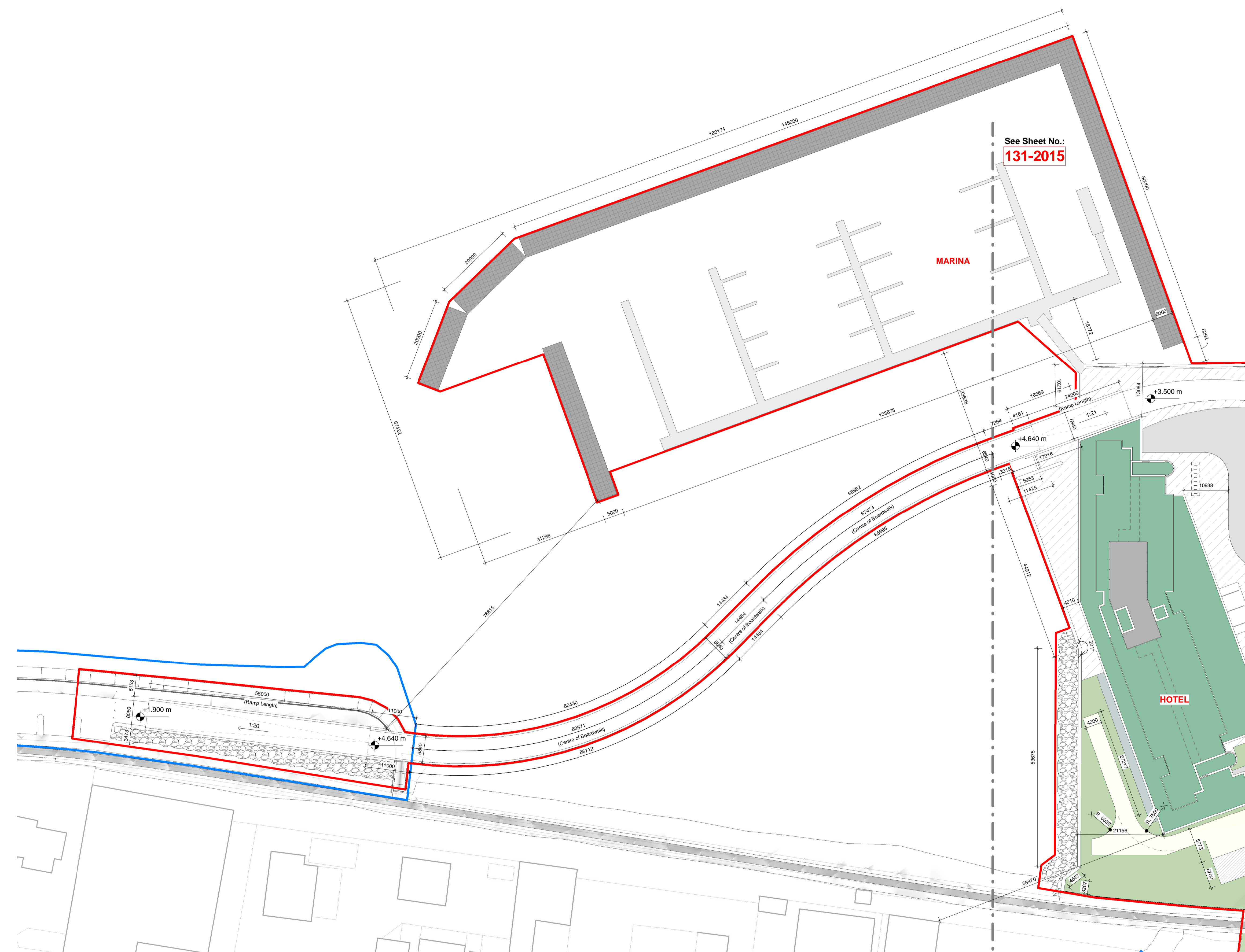
1-PROPOSED SITE LAYOUT - SITE DIMENSIONS - PAUL QUAY & BOARDWALK
